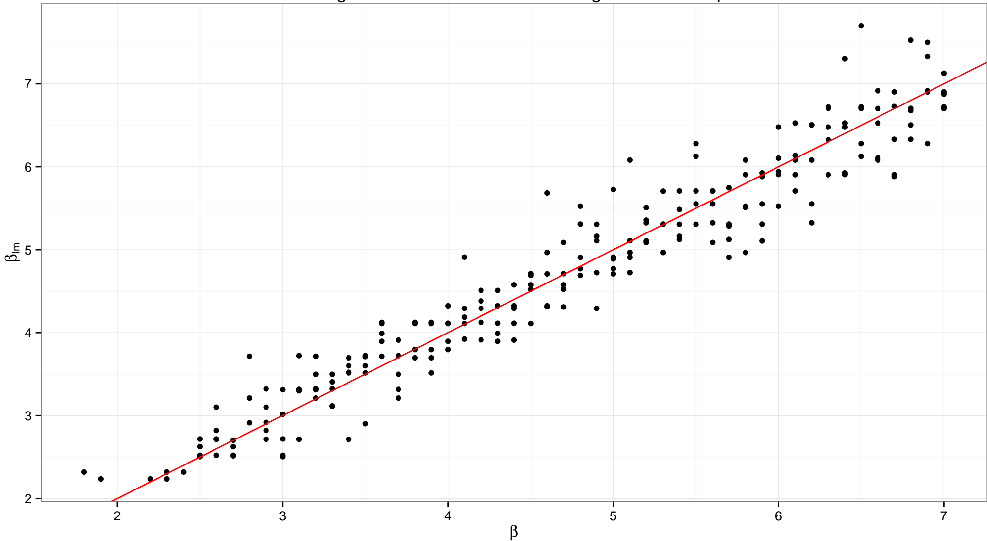
Predicting rate of infection on a network generated with p=0.5
